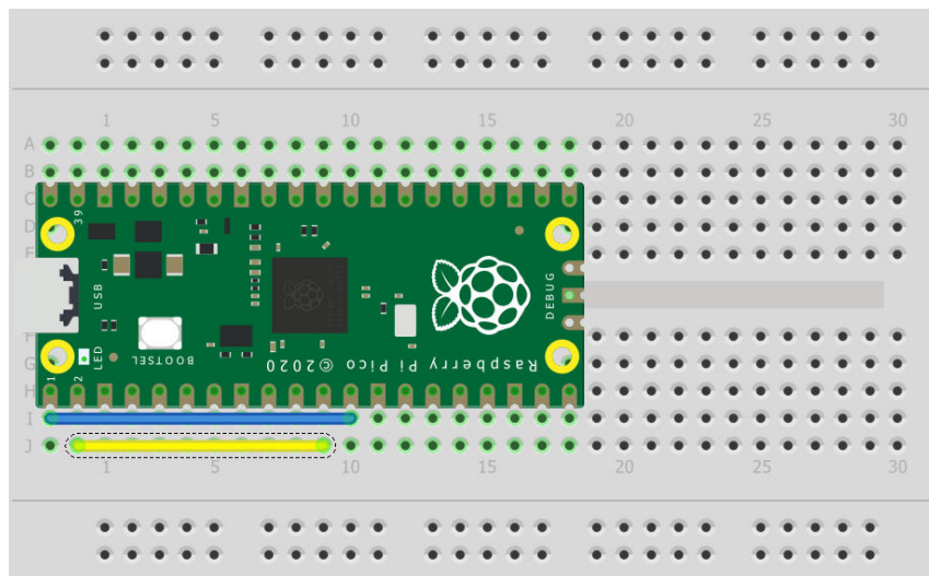
Figure 9. Wiring two of the Pico's ports together. Be sure to wire UART0 TX to UART1 RX and UART0 RX to UART1 TX.
